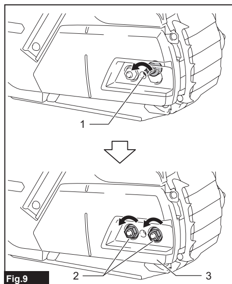
Fig.9 ► 1. Chain adjusting screw 2. Retaining nut 3. Sprocket cover
